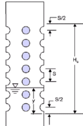
Perforated Riser Outlet Geosyntec Consultants
