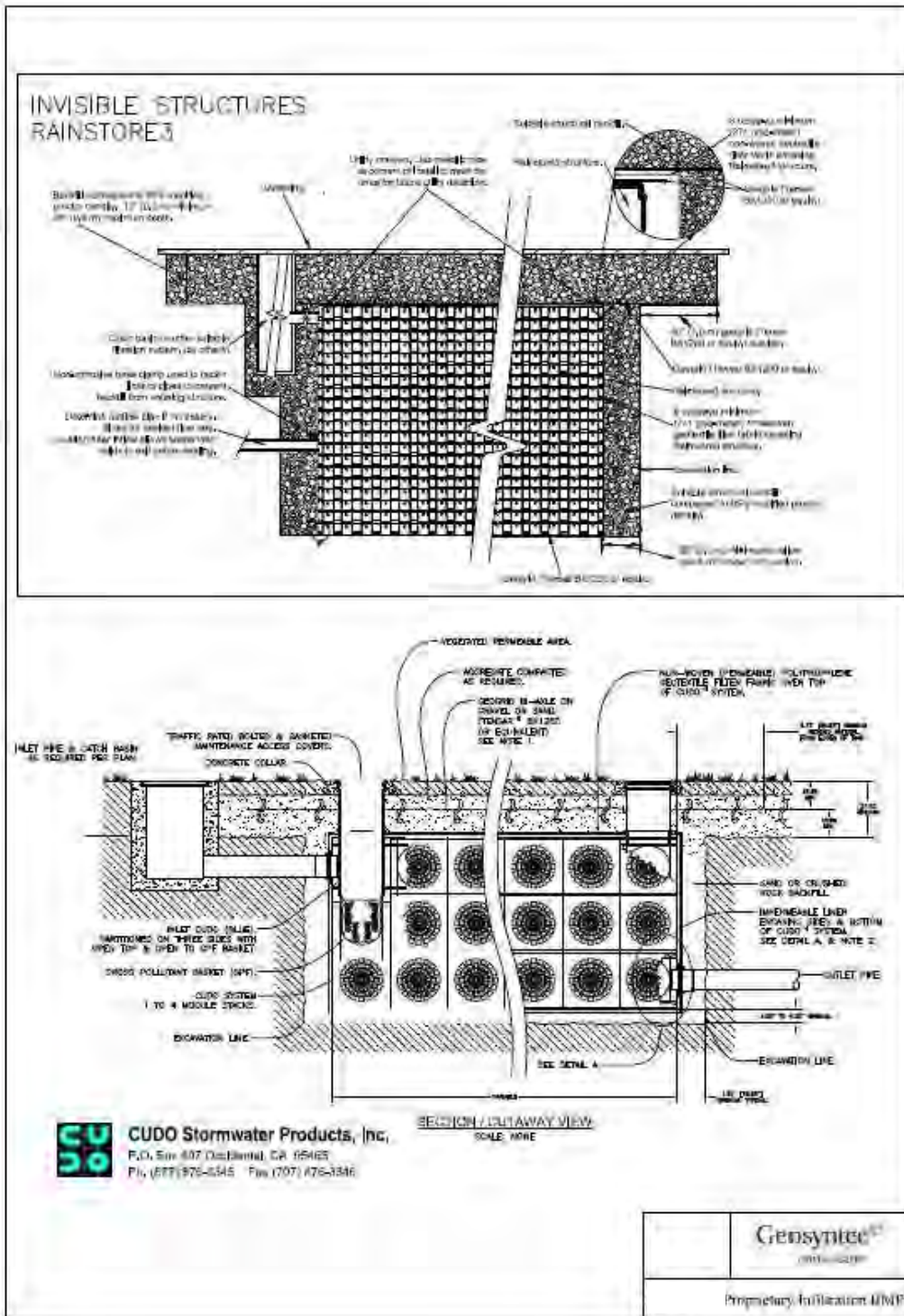
Figure 9. Subsurface Infiltration System (INF-6) Concept
