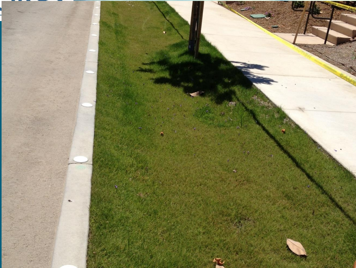
LID Parkway swale with zero curbs
