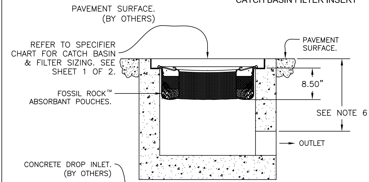
SECTION VIEW
