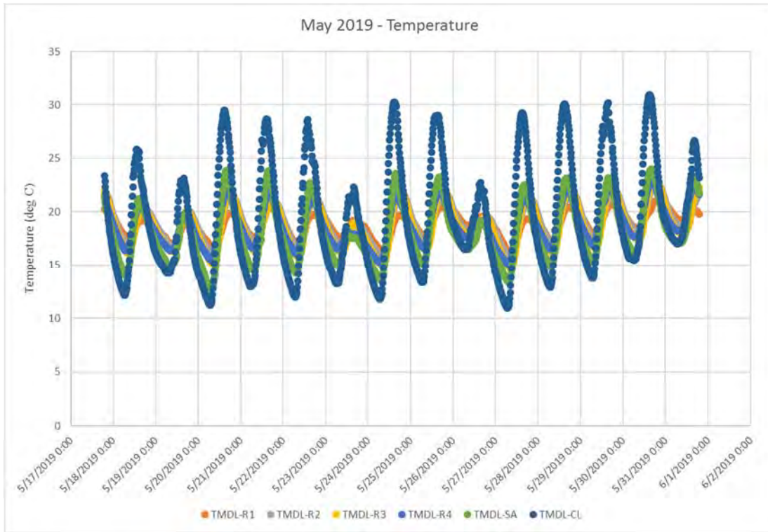
FIGURE 6. DRY SEASON 2019 - TEMPERATURE (CONTINUOUS DATA LOGGER)
