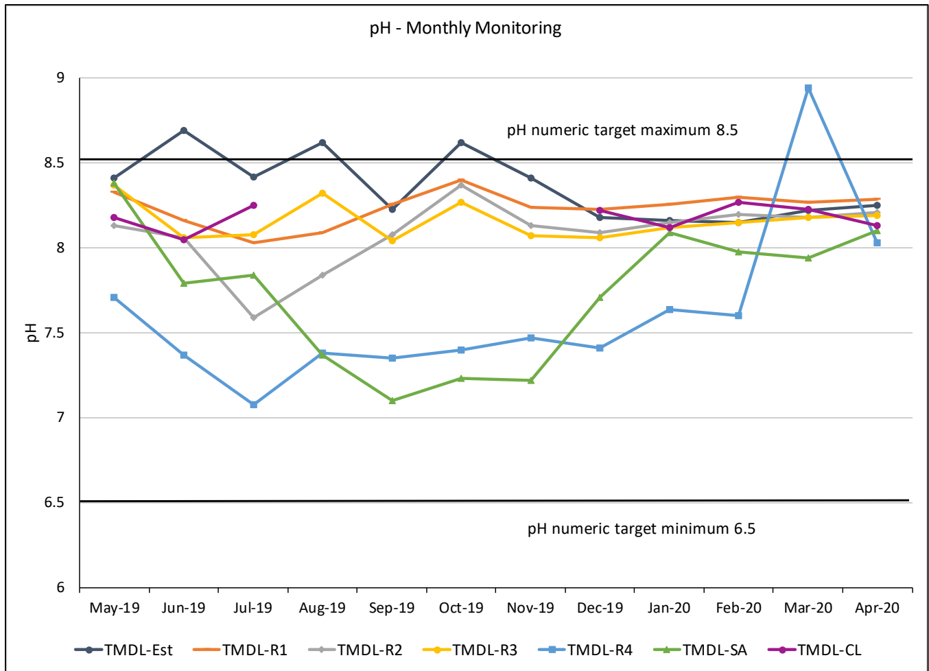
FIGURE 6. 2019 - 2020 MONTHLY MONITORING - PH
