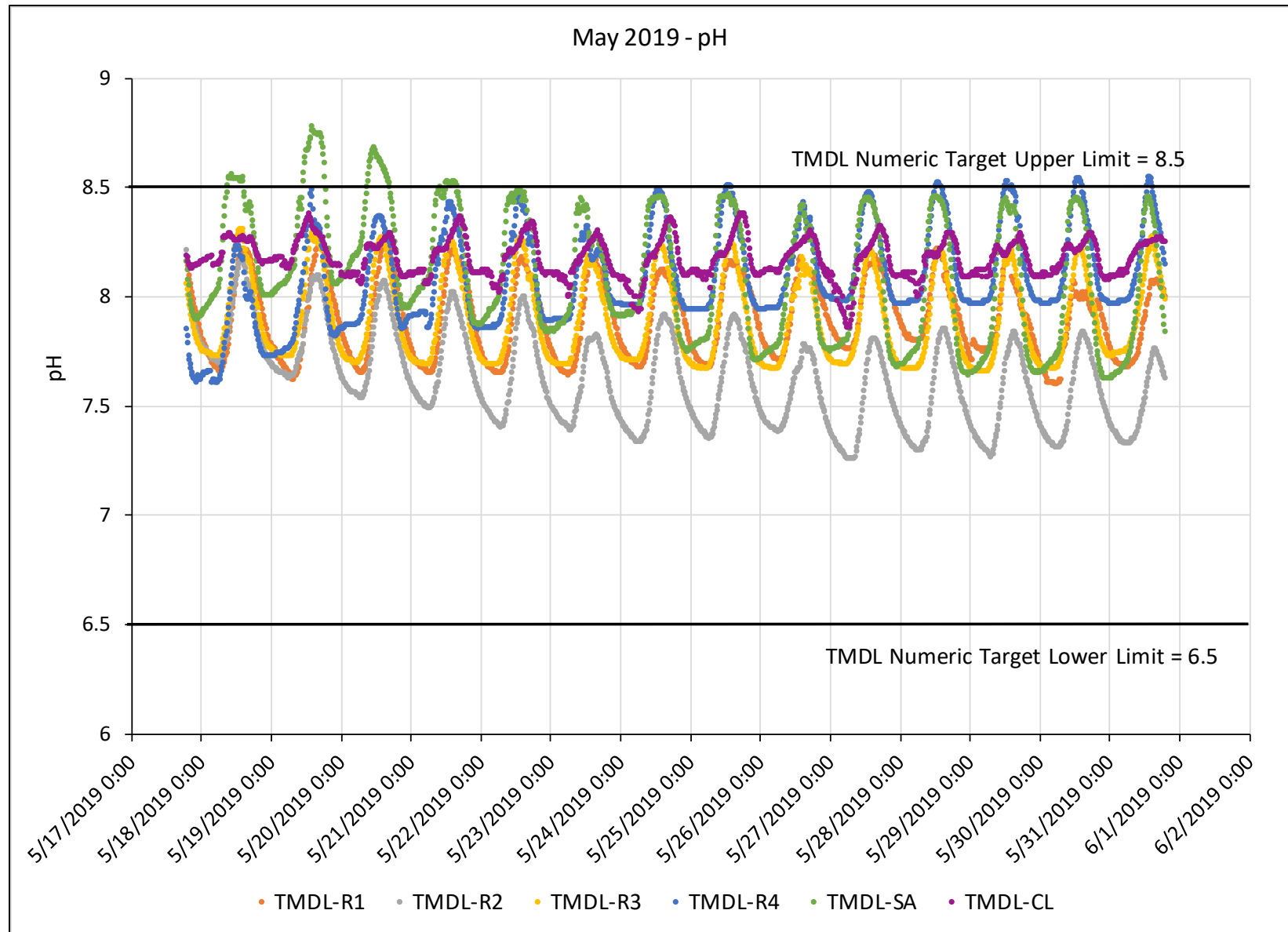
FIGURE D1. 2019 SECOND QUARTER PH CONTINUOUS DATA LOGGING
