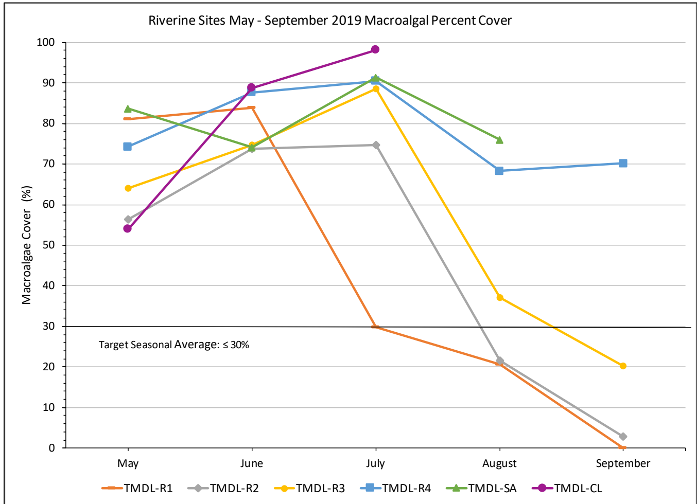
FIGURE 14. 2019-2020 DRY SEASON - MACROALGAL PERCENT COVER AT RIVERINE SITES
