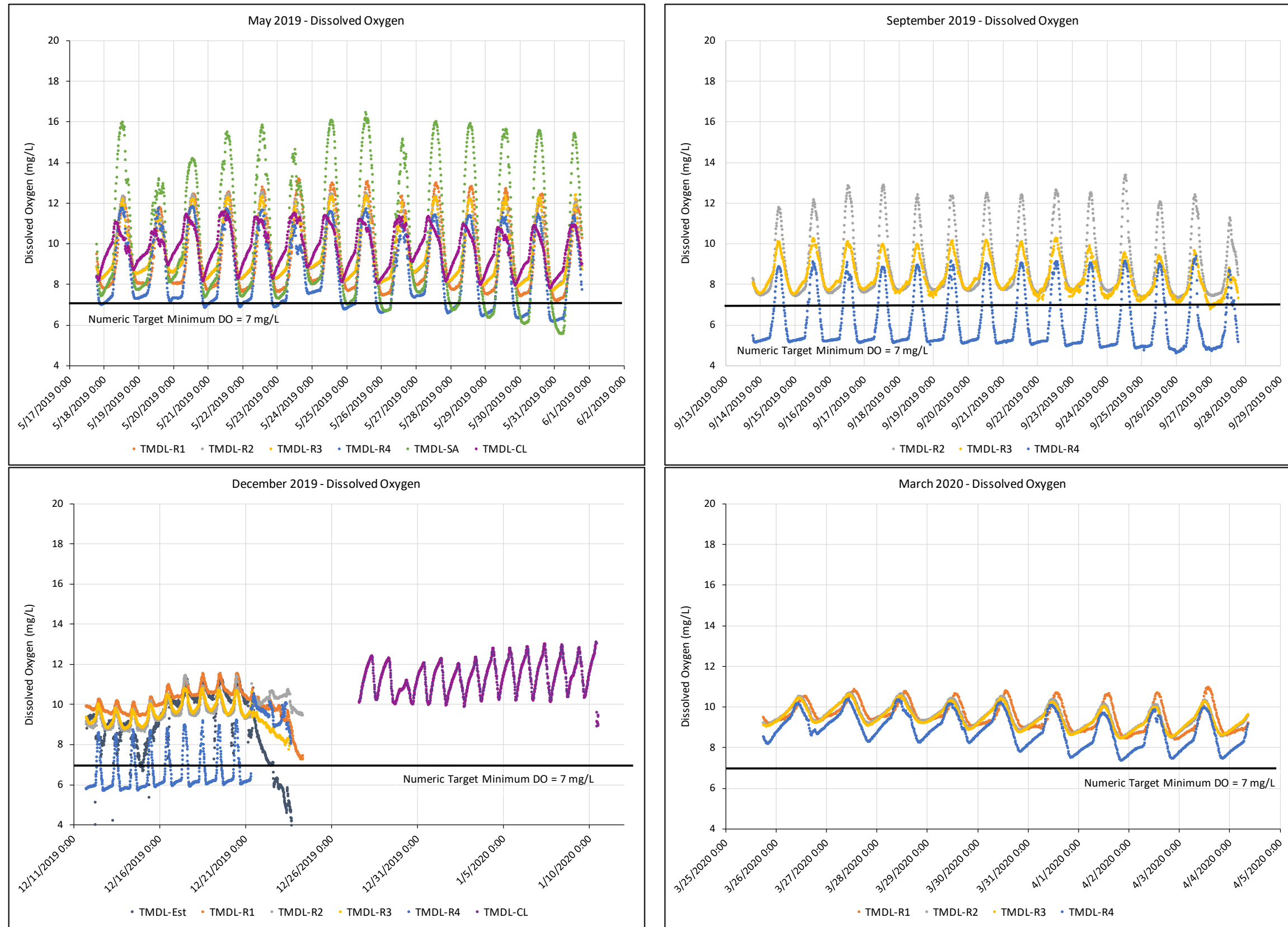
FIGURE 19. 2019-2020 CONTINUOUS DATA LOGGING – DISSOLVED OXYGEN
