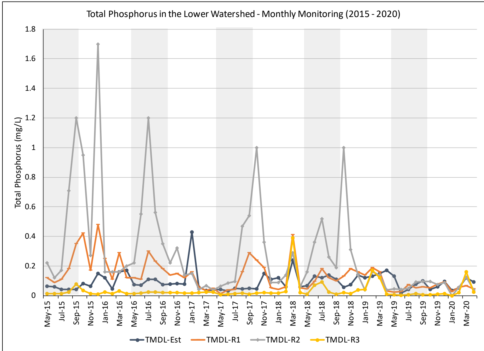
FIGURE 11. 2015 - 2020 MONTHLY MONITORING - TOTAL PHOSPHORUS, LOWER WATERSHED
