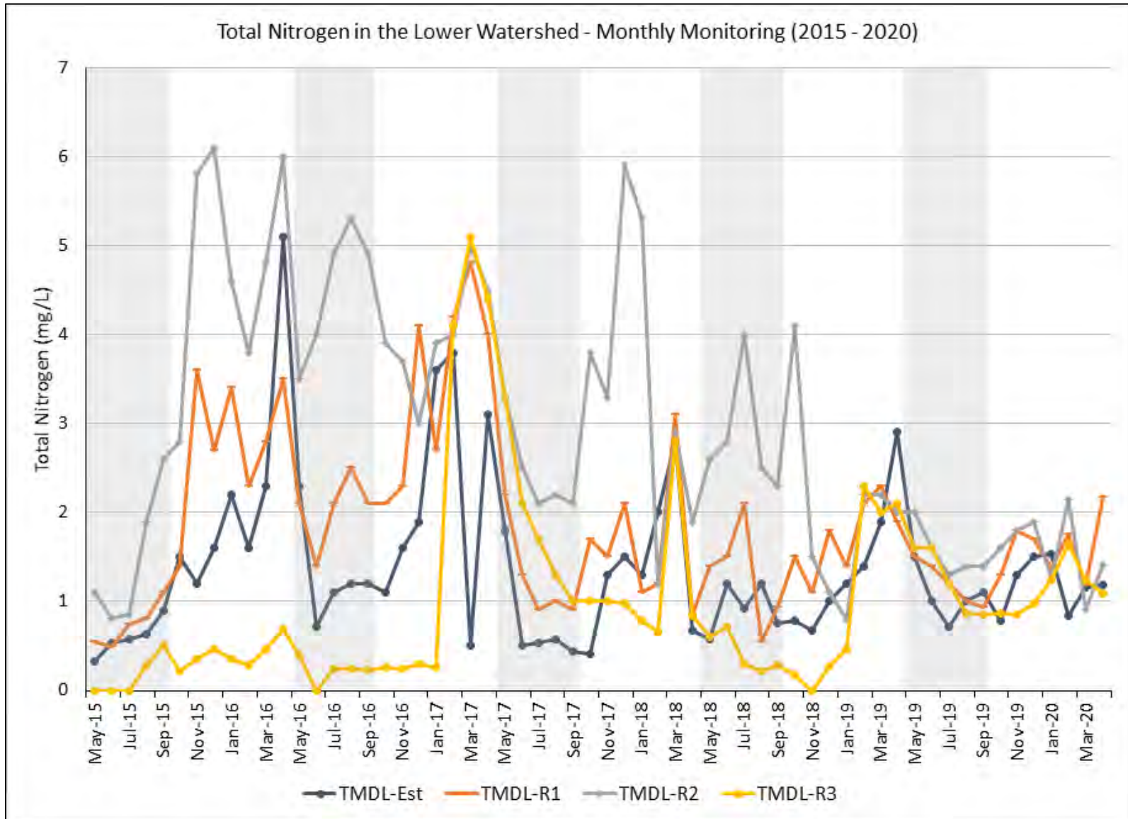
FIGURE 8. 2015 - 2020 MONTHLY MONITORING - TOTAL NITROGEN, LOWER WATERSHED
