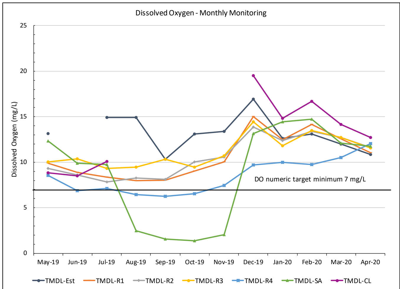
FIGURE 5. 2019 - 2020 MONTHLY MONITORING - DISSOLVED OXYGEN
