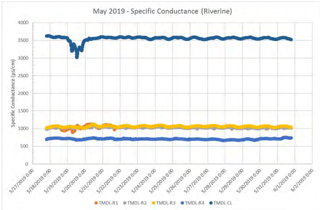
FIGURE 9. DRY SEASON 2019 - SPECIFIC CONDUCTANCE (CONTINUOUS DATA LOGGER)
