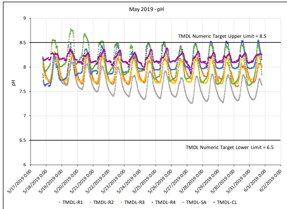
FIGURE 18. 2019-2020 CONTINUOUS DATA LOGGING – PH
