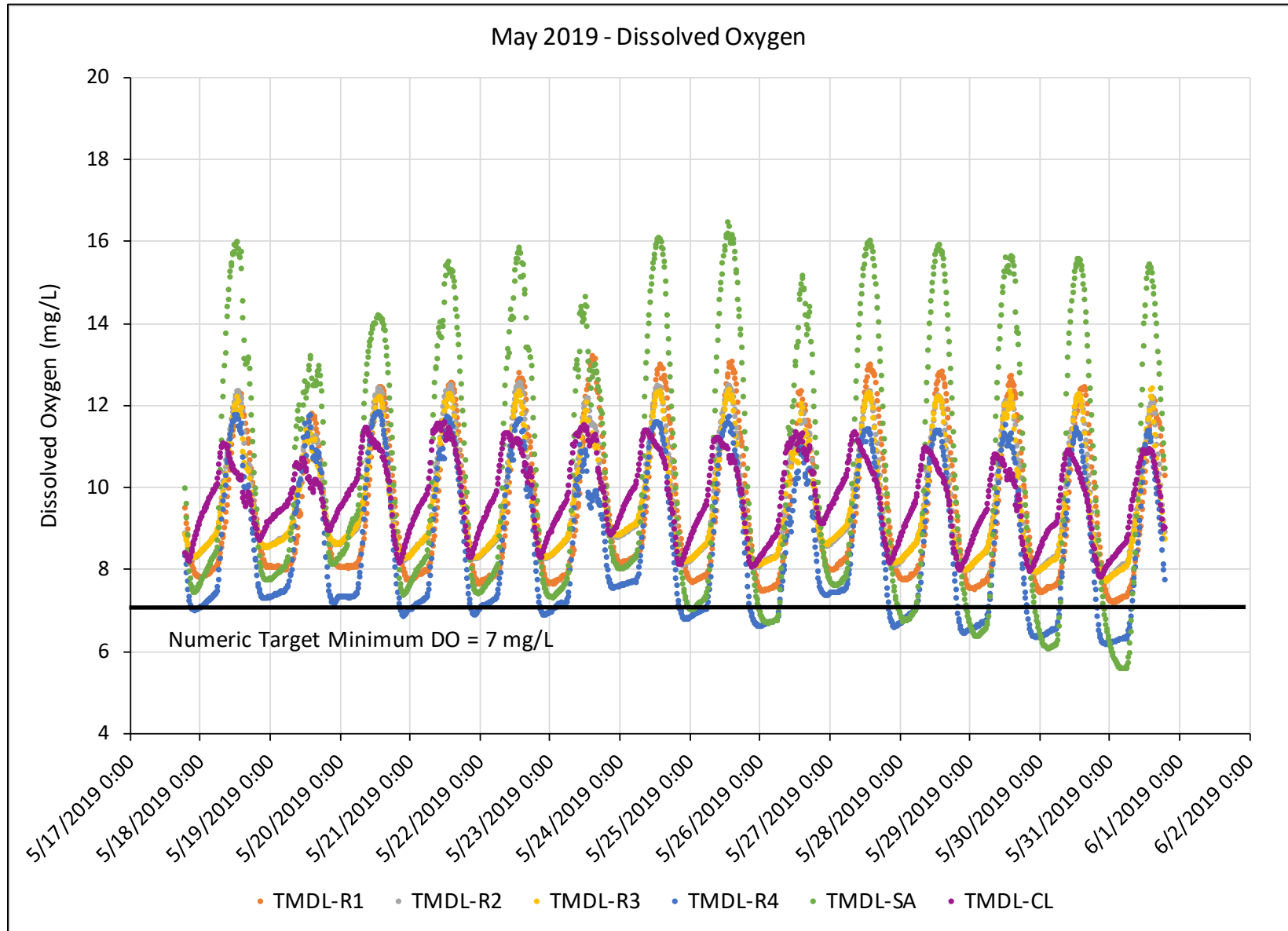
FIGURE D5. 2019 SECOND QUARTER DISSOLVED OXYGEN CONTINUOUS DATA LOGGING
