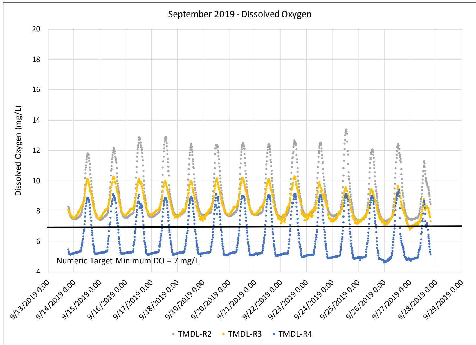
FIGURE D6. 2019 THIRD QUARTER DISSOLVED OXYGEN CONTINUOUS DATA LOGGING
