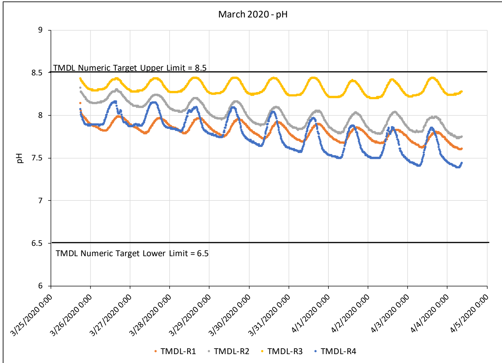
FIGURE D4. 2020 FIRST QUARTER PH CONTINUOUS DATA LOGGING
