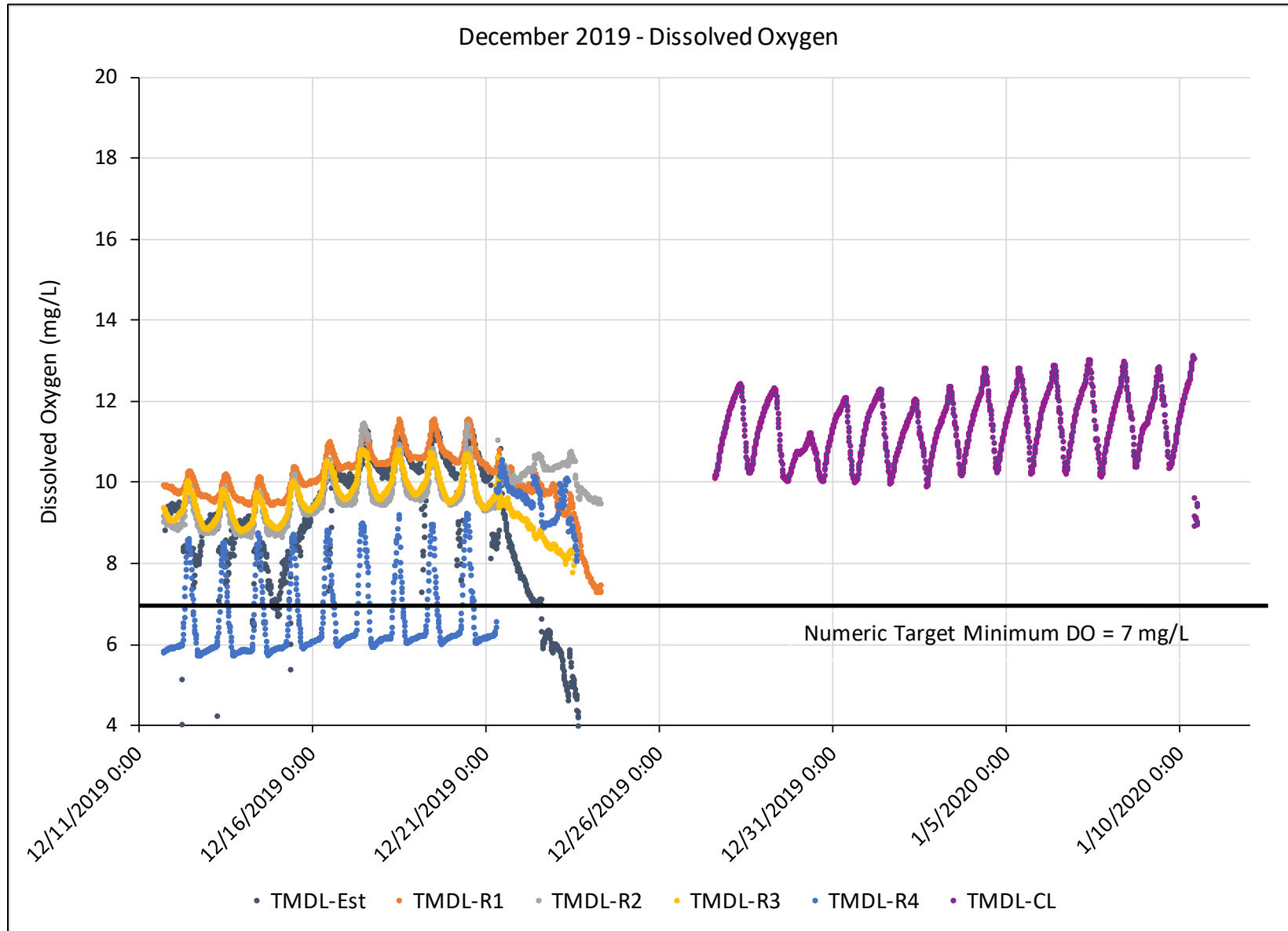
FIGURE D7. 2019 FOURTH QUARTER DISSOLVED OXYGEN CONTINUOUS DATA LOGGING
