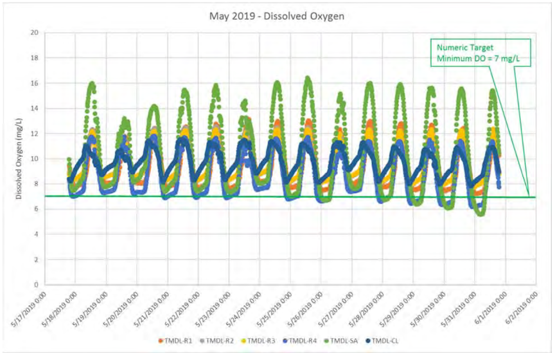
FIGURE 8. DRY SEASON 2019 - DISSOLVED OXYGEN (CONTINUOUS DATA LOGGER)
