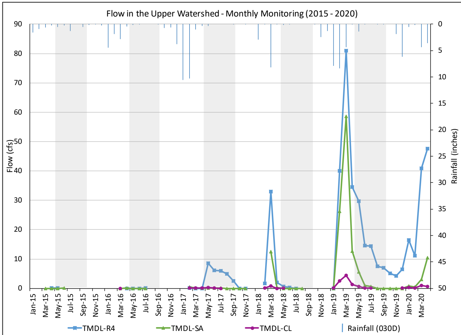
FIGURE 4. 2015-2020 MONTHLY FLOW MONITORING IN THE UPPER WATERSHED
