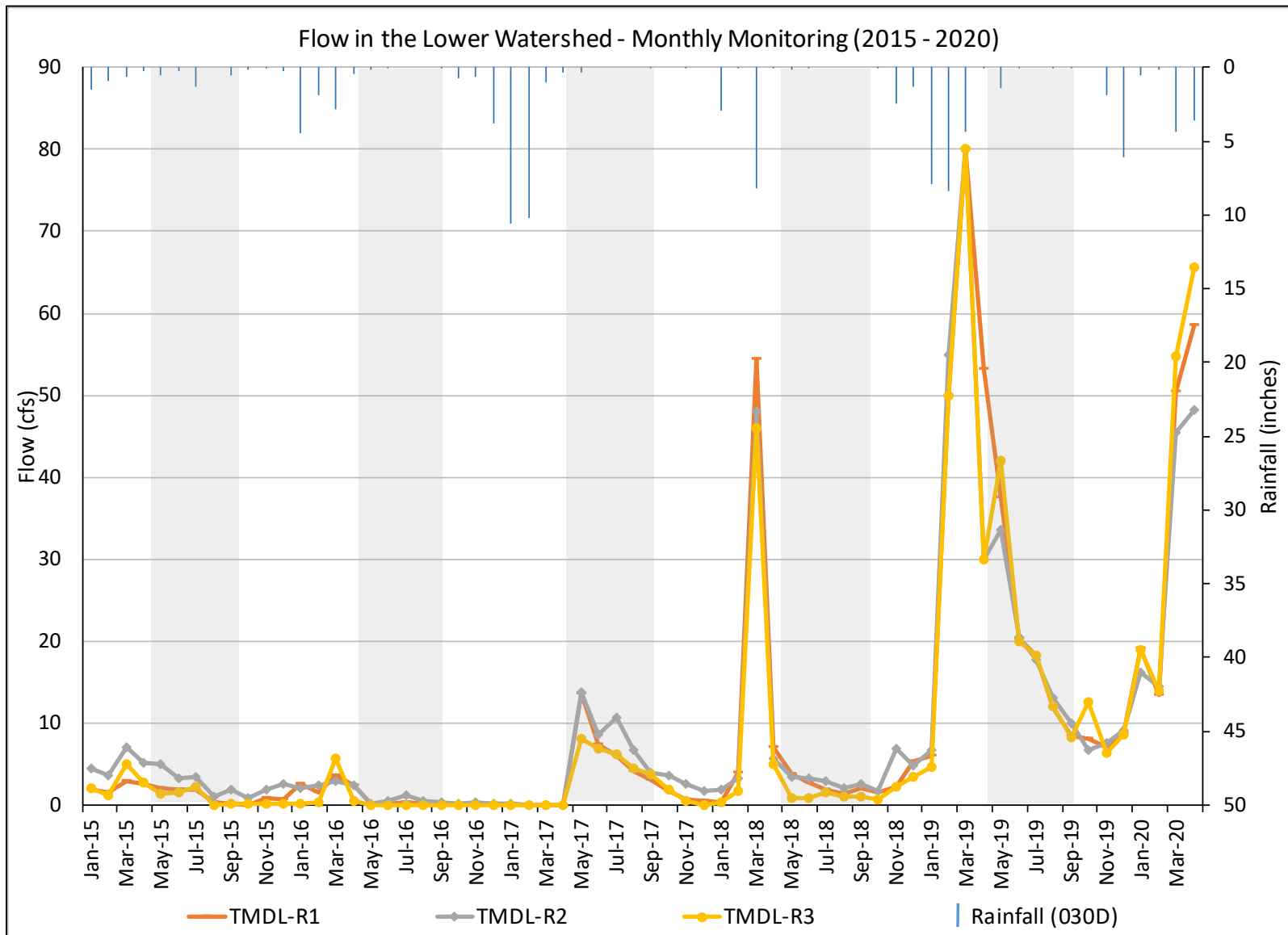
FIGURE 3. 2015-2020 MONTHLY FLOW MONITORING IN THE LOWER WATERSHED
