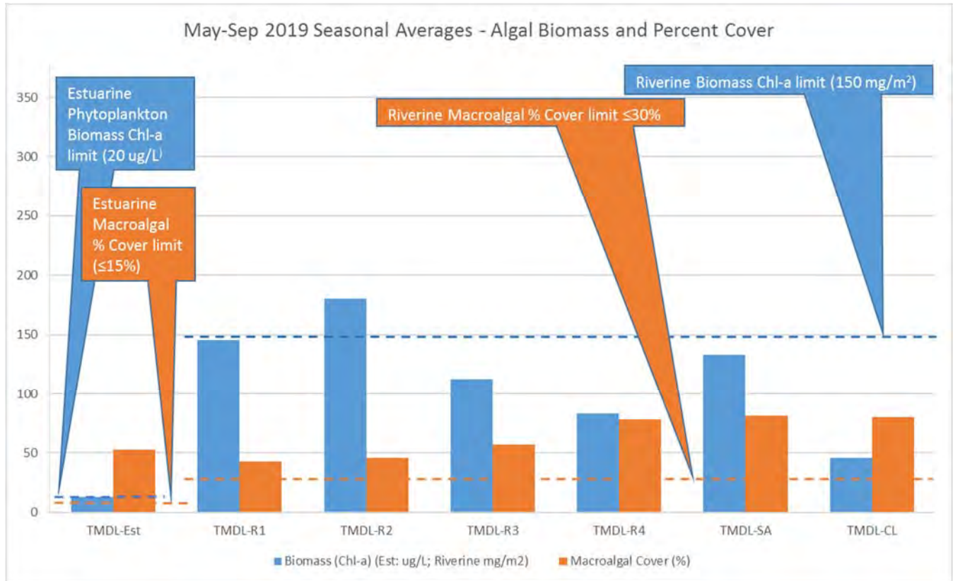
FIGURE 4. DRY SEASON SEASONAL AVERAGES - CHLOROPHYLL A AND MACROALGAL COVER
