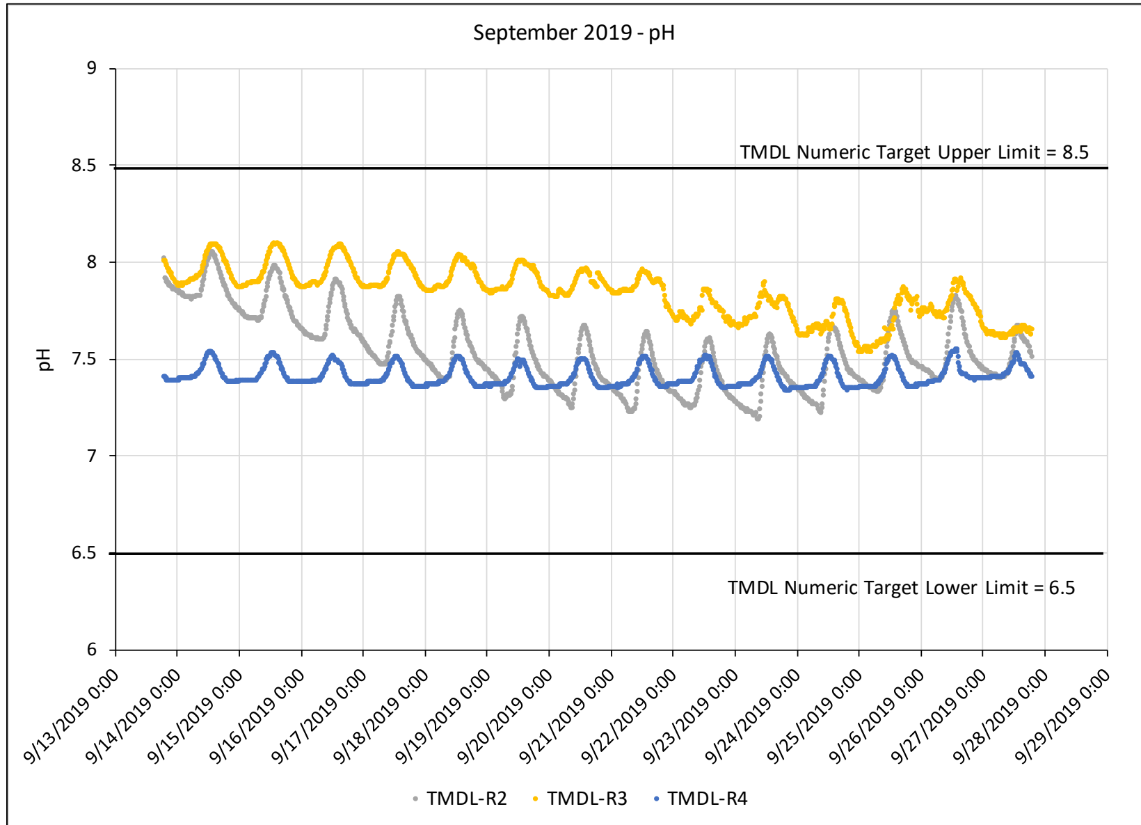
FIGURE D2. 2019 THIRD QUARTER PH CONTINUOUS DATA LOGGING
