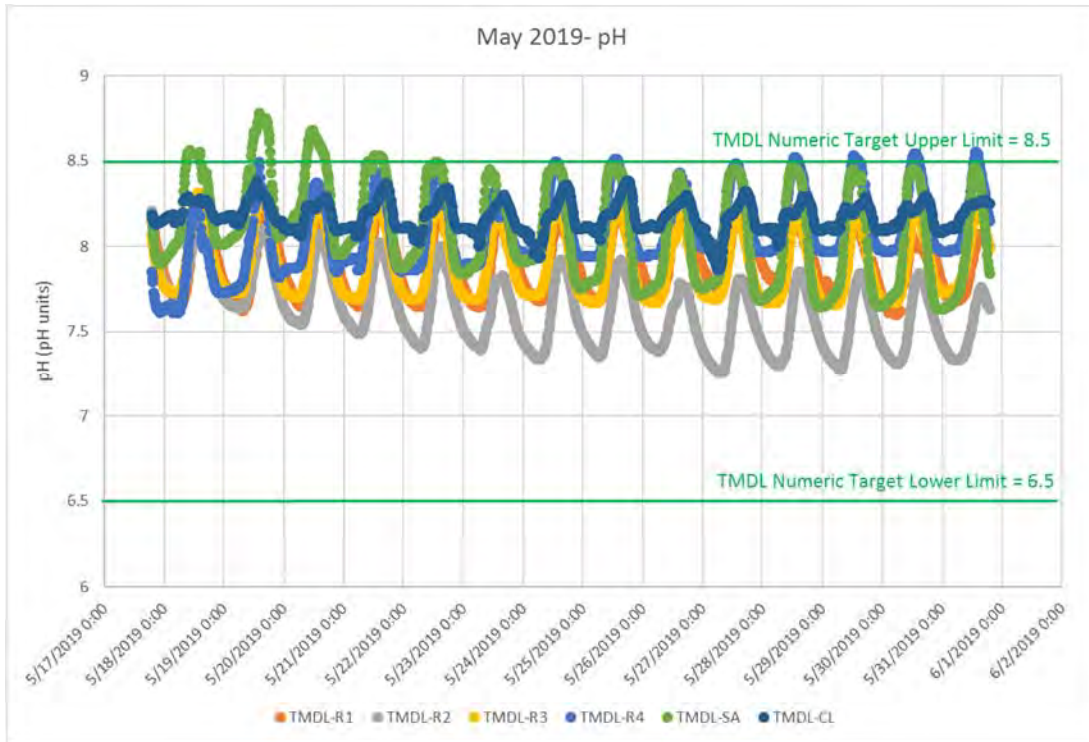
FIGURE 7. DRY SEASON 2019 - PH (CONTINUOUS DATA LOGGER)
