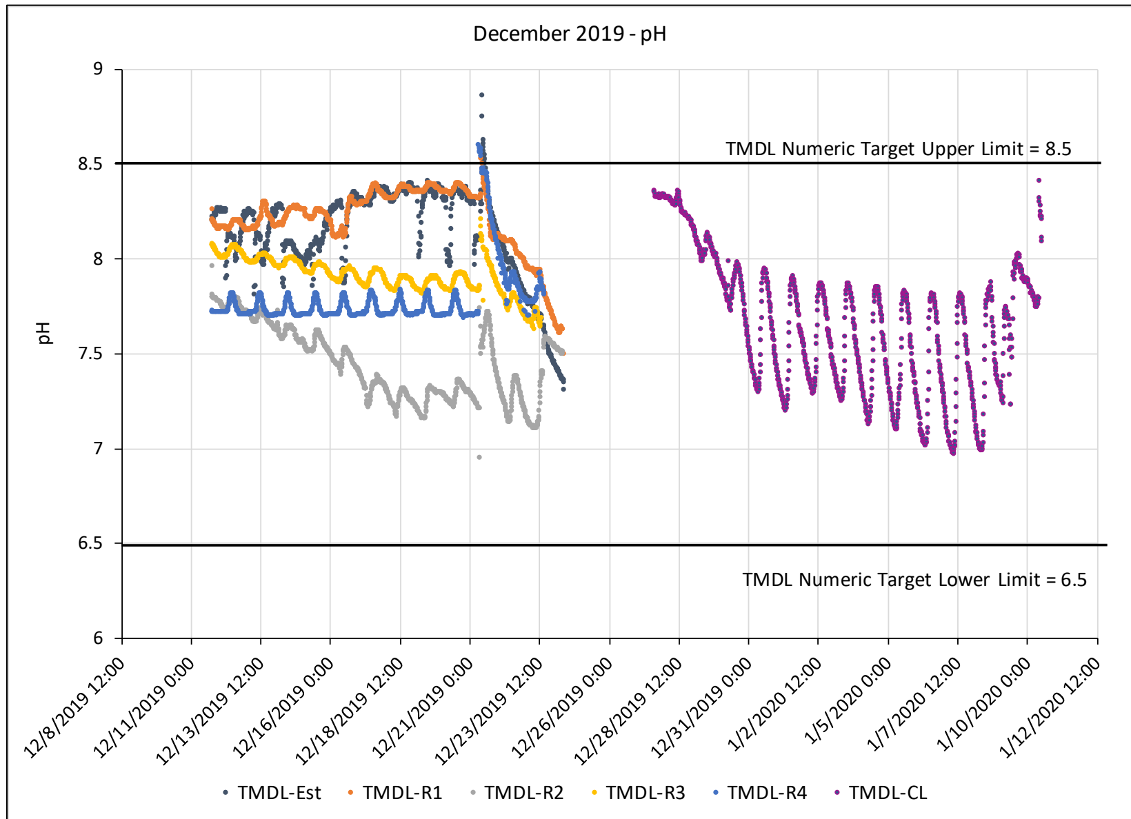
FIGURE D3. 2019 FOURTH QUARTER PH CONTINUOUS DATA LOGGING
