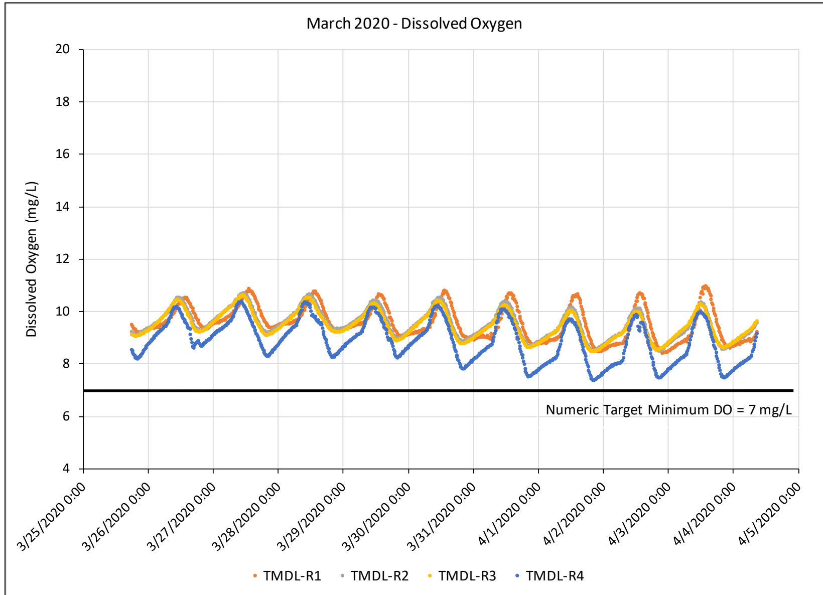
FIGURE D8. 2020 FIRST QUARTER DISSOLVED OXYGEN CONTINUOUS DATA LOGGING
