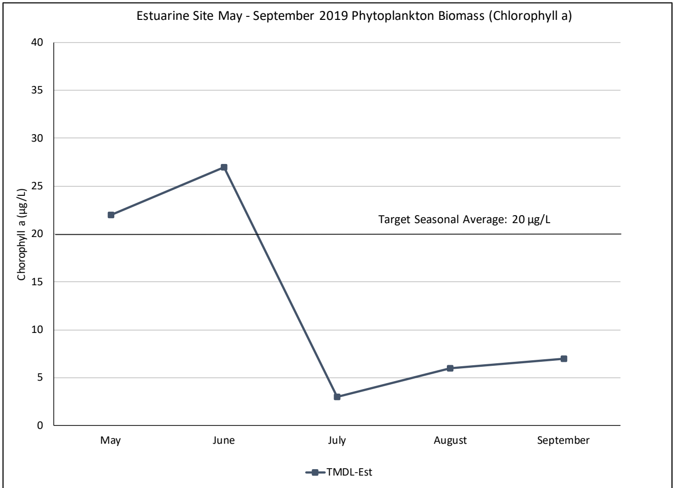
FIGURE 15. 2019-2020 DRY SEASON – ESTUARY CHLOROPHYLL A
