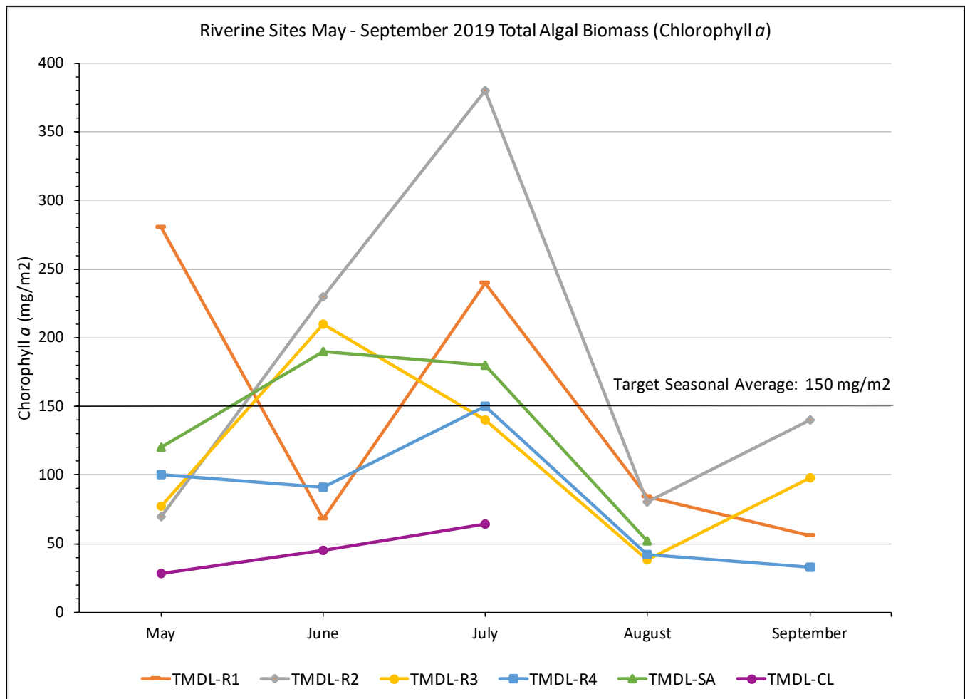
FIGURE 13. 2019-2020 DRY SEASON - TOTAL ALGAL BIOMASS (CHLOROPHYLL A) AT RIVERINE SITES
