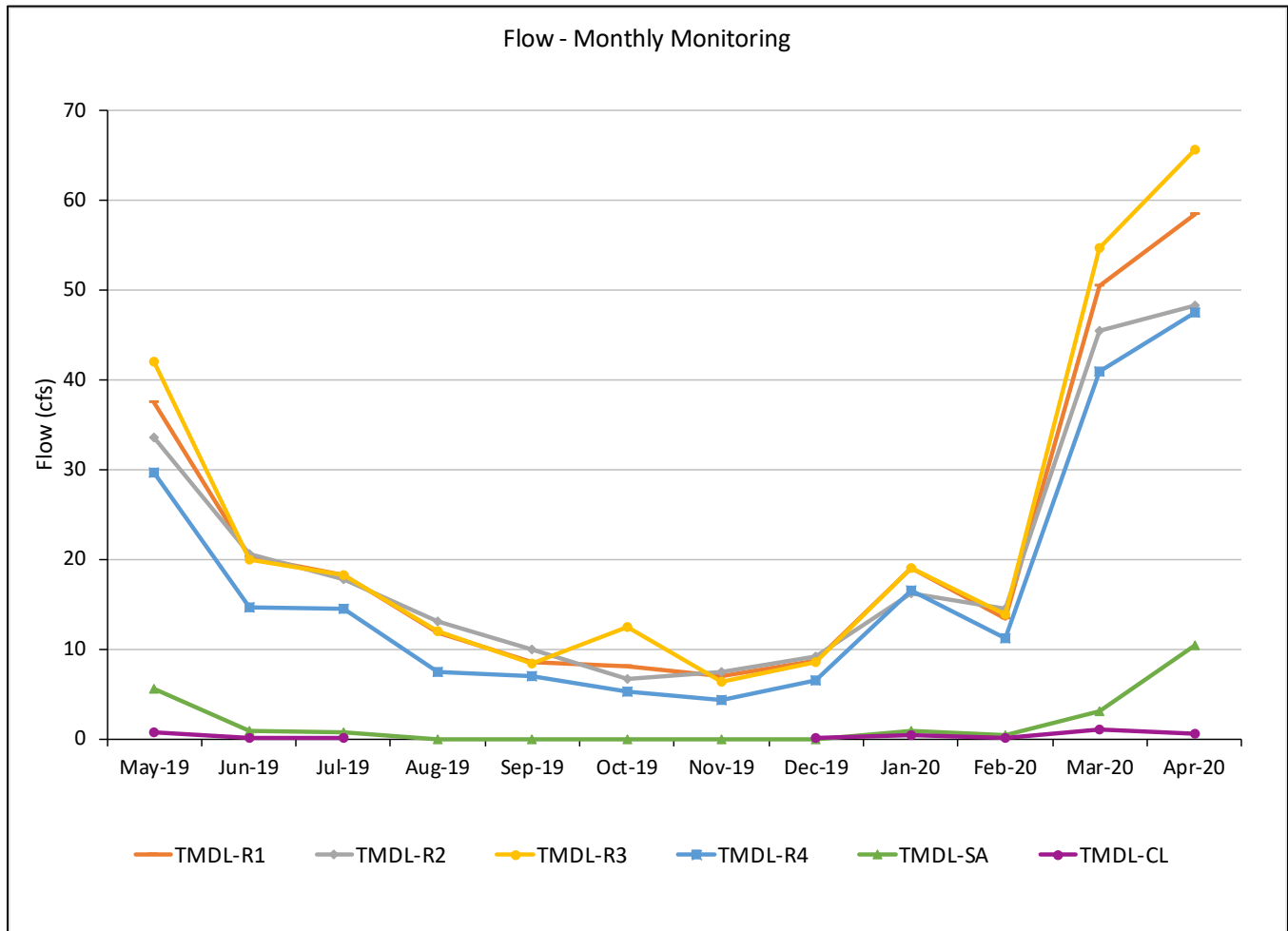
FIGURE 2. 2019-2020 MONTHLY FLOW MONITORING
